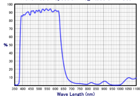
Transmission Spectrum Magnitude of MFC65
